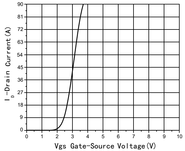
Fig2 Transfer Characteristics
