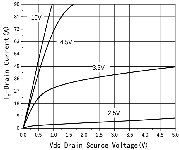
Fig1 Output Characteristics
