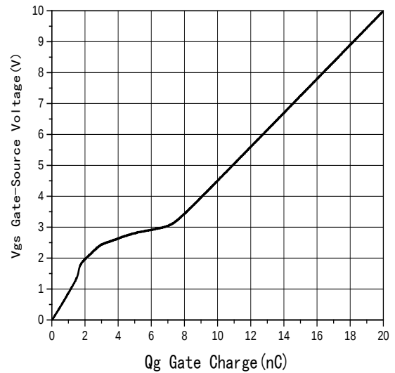
Fig6 Gate Charge
