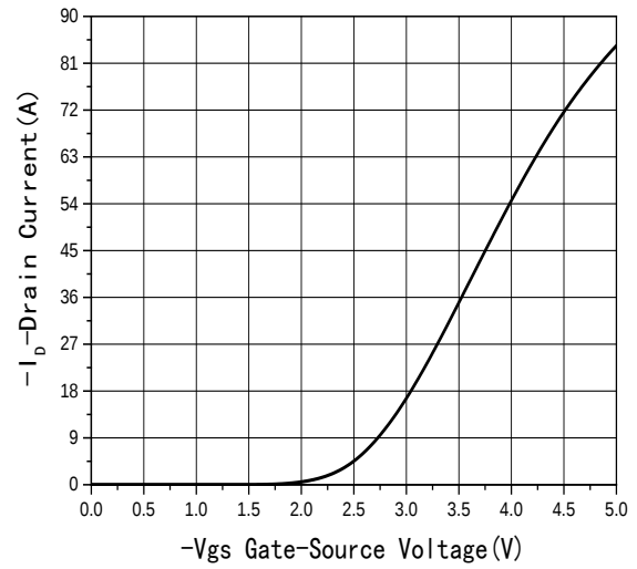
Fig2 Transfer Characteristics
