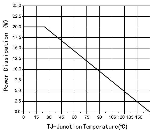
Fig7 Power De-rating
