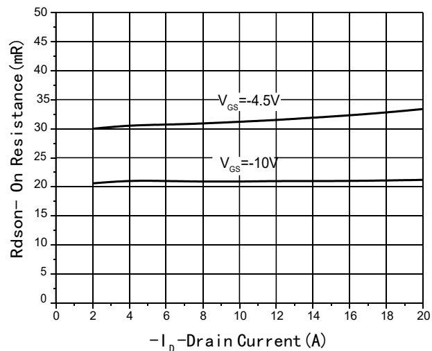
Fig3 Rdson-Drain current
