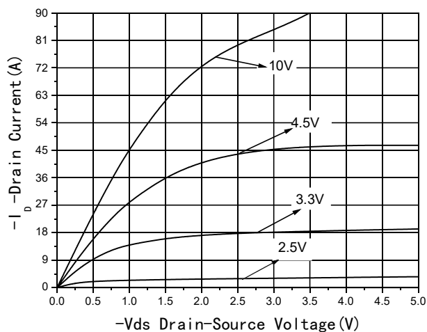
Fig1 Output Characteristics
