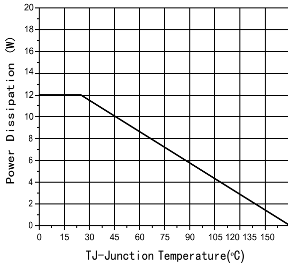
Fig7 Power De-rating
