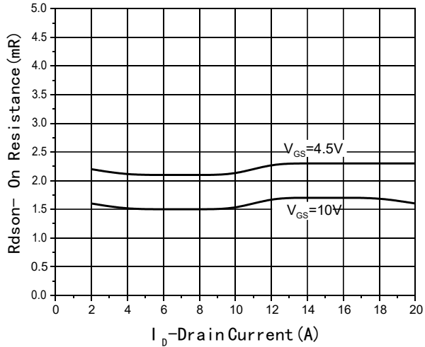
Fig3 Rdson-Drain current
