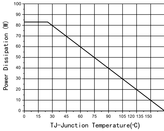
Fig7 Power De-rating
