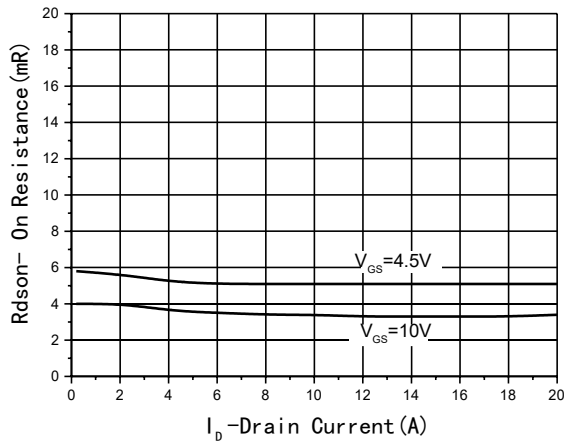
Fig3 Rdson-Drain current
