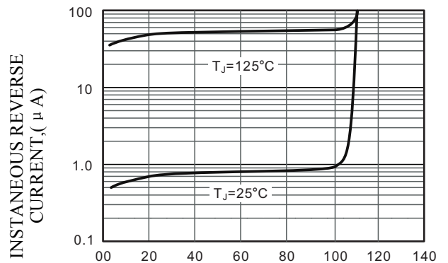
FIG.4-TYPICAL REVERSE CHARACTERISTICS
